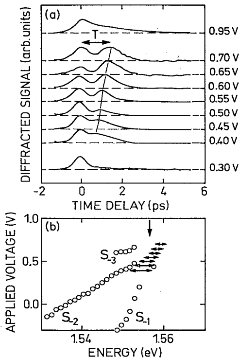
FIG. 1. (a) DFWM signal vs time delay between the two exciting laser pulses for several voltages in the WS ladder regime, showing modulations of period T . (b) The peak positions of "oblique" transitions are plotted as circles vs the applied voltage. The energy intervals h/T , with T from (a), are shown as horizontal arrows.
