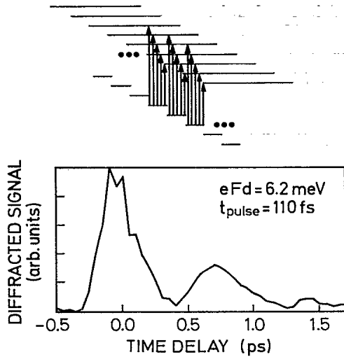
FIG. 2. DFWM signal vs time delay for eFd = 6.2 meV using 110-fs laser pulses. Under this condition, optical transitions from each localized hh state to about five conduction-band WS states takes place as illustrated in the upper part.
