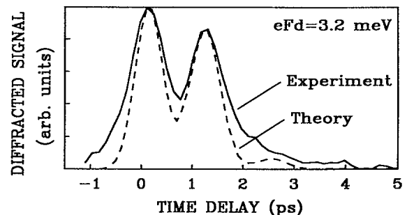
FIG. 3. Experimentally determined DFWM signal for an applied voltage of 0.55 V (solid line) together with the calculated DFWM curve (dashed line) using the experimental parameters as described in the text.
