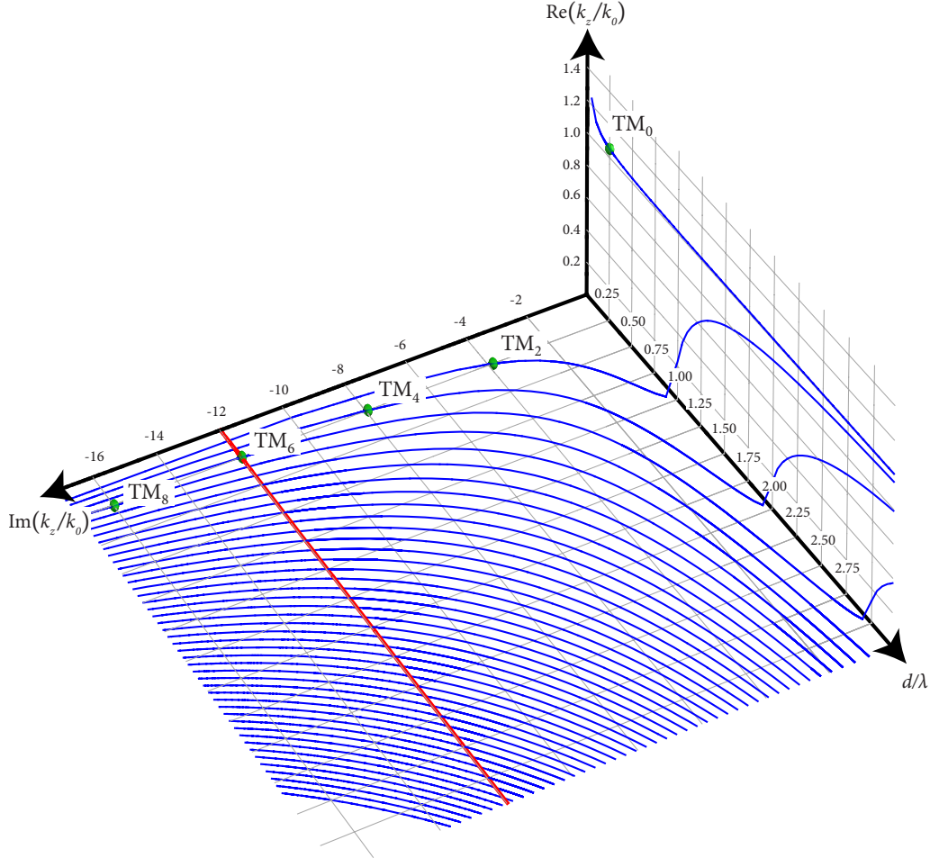
FIG. 5. (Color online) Spectrum of the MIM waveguide as a function of d=2a , \text{Re}(k_z/k_0) , and \text{Im}(k_z/k_0) , where k_0=2\pi/\lambda is the free space wave vector. \epsilon_m=-143.497 is assumed, which corresponds to the real part of the permittivity of silver at a wavelength of \lambda=1550 nm. The thick line denotes the limit of the real spectrum. Spheres denote the point spectrum for the d=2a=\lambda/4 case as also shown in Fig. 4. It can be seen that only the lowest-order mode, \text{TM}_0 , is propagating for d=\lambda/4 and the rest of the modes are highly evanescent.
