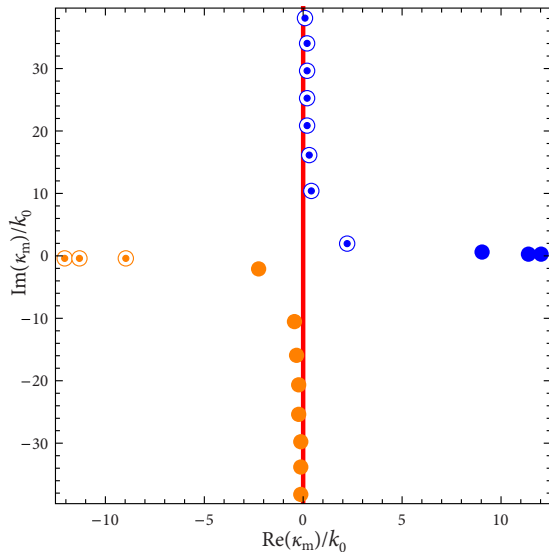
FIG. 7. (Color online) Effects of loss on the spectrum. All parameters are the same as in Fig. 6 except \epsilon_m = -143.497 - i9.517 . Comparison with Fig. 6 shows that the forward, proper, complex modes on the fourth quadrant have moved to the third quadrant and thus became leaky modes.
