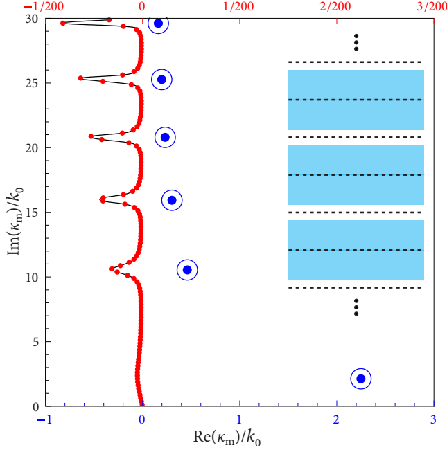
FIG. 9. (Color online) Effects of termination of the metal by a PEC wall—as in Fig. 8—on the spectrum. \epsilon_m = -143.497 - i9.517 , \epsilon_i = 1.0 , 2a = \lambda/4 , h = 2\lambda , k_0 = 2\pi/\lambda , and \lambda = 1550 nm. The spectrum looks very similar to Fig. 7. In order to highlight the discretization of the continuum, we show a zoomed portion of the \kappa_m plane. The complex modes and the discretuum show anticrossing behavior. We use two different axes for the real part of \kappa_m . The scale on the bottom refers to the complex modes, \odot , whereas the one on the top refers to the discretuum, \bullet . The inset shows a portion of the infinite lattice created by the repeated application of image reflection off of the PEC boundaries. Dashed lines in the inset signify the locations of zero tangential electric field, where a PEC termination can be applied. In separate calculations not shown in this figure, we observe that as h is increased, the magnitude of the anticrossing behavior of the continuum decreases as a result of decreased coupling between adjacent MIM waveguides.
