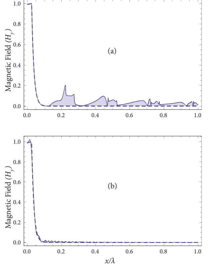
FIG. 10. (Color online) Effects of the continuous spectrum on mode expansion. \epsilon_m = -143.497 - i9.517 . The main mode of the right waveguide, h_R^{(1)}(x) , with 2a' = \lambda/20 is expanded in terms of the modes of the left waveguide, h_L^{(m)}(x) , with 2a = \lambda/4 . The dashed lines show the magnitude of the magnetic field profile of the main mode of the right waveguide. The solid line shows the result of the expansion of Eq. (17). Shaded regions show the error from the use of a particular expansion and the actual right waveguide mode. Due to symmetry, only half of the full modal profile is plotted. (a) Open waveguide of Fig. 3, expansion made using the point spectrum only. (b) PEC terminated MIM waveguide of Fig. 8, with a+h=a'+h'=\lambda , expansion made using the discretuum and the point spectrum.
