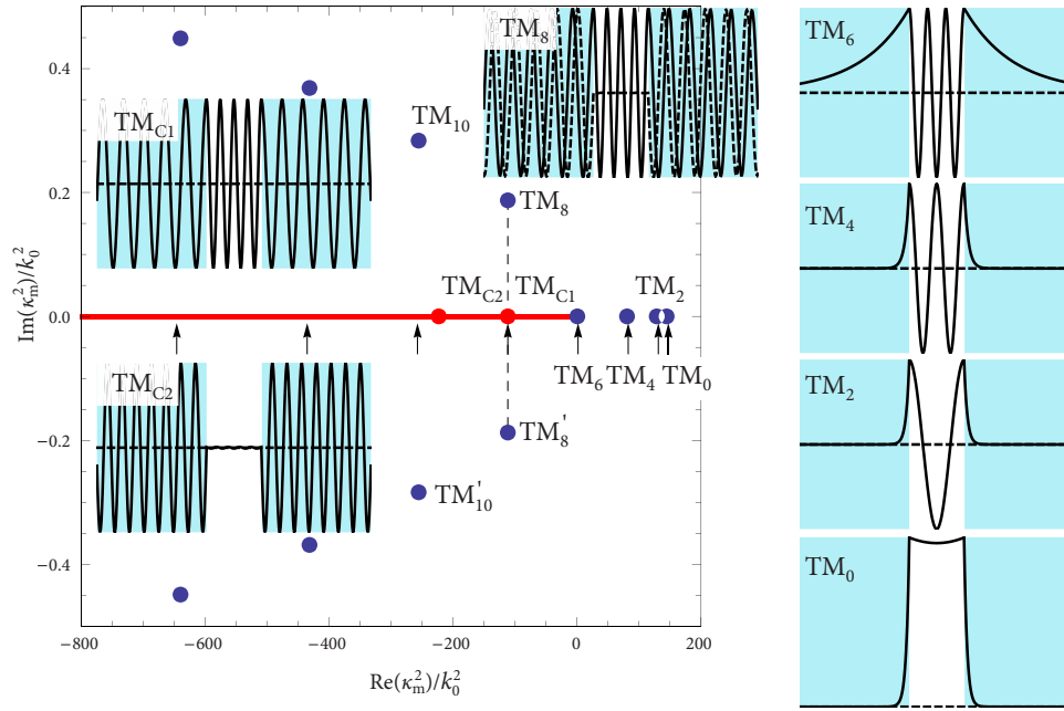
FIG. 4. (Color online) Spectrum of the MIM waveguide for \epsilon_m = -143.497 and 2a = \lambda/4 , where \lambda = 1550 nm is the wavelength of operation. There are four real modes and an infinite number of complex modes, all denoted with the \bullet symbol. The thick line denotes the continuous spectrum. Due to the fact that \epsilon_m is real, complex modes come in complex-conjugate pairs. Insets show the H_y mode shapes in the x direction for the discrete spectrum ( TM_0 through TM_8 ) and the continuous spectrum ( TM_{C1} and TM_{C2} )— solid lines in the insets are the real part of the mode, dashed lines are the imaginary part. The locations of the drawn continuous modes are shown by the \bullet symbol. Modes in the continuous spectrum are purely oscillatory in the x direction. Complex modes have a small decay, which is not visually apparent in the inset for TM_8 . Arrows ( \uparrow ) denote the position of the modes of a parallel-plate waveguide with a separation of a —equivalent to the limiting case h \rightarrow 0 in Fig. 8.
