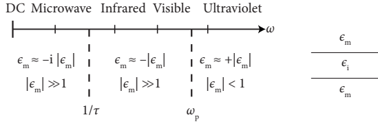
FIG. 1. The change in the metallic permittivity ( \epsilon_m ) as the frequency of operation ( \omega ) is varied leads to an evolution from the parallel-plate waveguide at low frequencies to the dielectric slab waveguide at high frequencies for the two-dimensional metal-insulator-metal geometry. We are assuming that \epsilon_m is a Drude model metal, where \tau is the average time between collisions among the ions of the lattice and the free electrons, and \omega_p is the plasma oscillation frequency.
