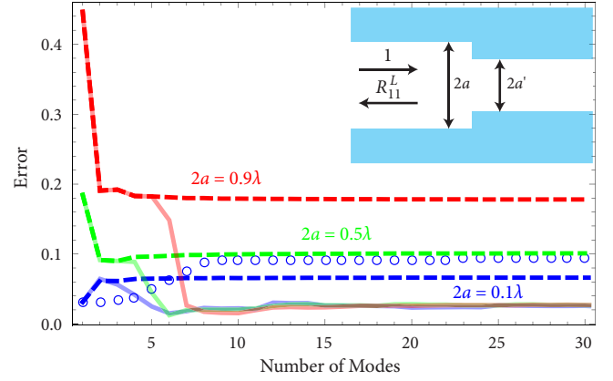
FIG. 11. (Color online) Convergence study of the reflection coefficient, R_{11}^L , of the main mode of the left waveguide traveling toward the right waveguide for 2a=0.9\lambda , 2a=0.5\lambda , and 2a=0.1\lambda . a'/a=0.4 and \epsilon_m=-143.497-i9.517 for all cases. Dashed lines are for calculations including the point spectrum only. Solid lines are those with both the point and the continuous spectrum. Empty circles denote the calculations done with the forward point spectrum and the continuous spectrum for the 2a=0.1\lambda case only. Error is defined as |(R_{11}^{L,MM} - R_{11}^{L,FDFD})/R_{11}^{L,FDFD}| , where MM stands for mode matching and FDFD for finite-difference frequency-domain calculations. The inset shows the junction geometry.
