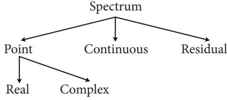
FIG. 2. Classification of the spectrum for an operator in a general space. Point spectrum is sometimes called the discrete spectrum.
