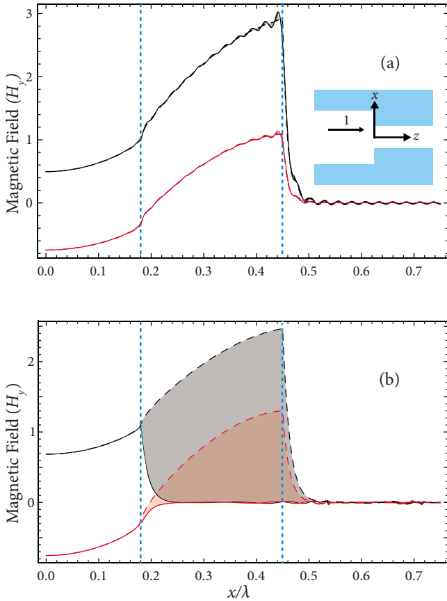
FIG. 12. (Color online) Magnetic field H_y at the junction of two MIM waveguides as a result of the scattering of the main mode of the left waveguide traveling toward the right—the inset shows the schematic of the geometry. The left waveguide has 2a=0.9\lambda , the right waveguide has 2a'=0.36\lambda so that a'/a=0.4 as in Fig. 11. a+h=a'+h'=3\lambda/4 . Fields on the left of the junction are dashed, fields on the right are shown with solid lines for both the real and the imaginary part of the magnetic field profile. The difference between the left and right fields is shaded. Due to symmetry, only half of the field profile is plotted. Vertical dotted lines at x=0.18\lambda and x=0.45\lambda denote the end of the insulator region for the right and the left side of the junction, respectively. (a) Mode-matching calculations using the point and the continuous spectrum—60 modes in total—showing good agreement between the fields just on the left and just on the right of the junction. (b) Mode-matching calculations using the point spectrum only—100 modes in total—showing clear disagreement between the calculated fields just on the left and just on the right of the junction.
