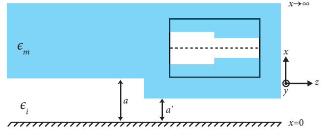
FIG. 3. (Color online) Geometry for the even modes of the MIM waveguide. The x=0 plane contains a fictitious perfect electric conductor to simplify the problem when dealing only with even TM modes of the guide. This fictitious MIM waveguide is equivalent to an actual guide with an insulator thickness of 2a . The inset shows the equivalent symmetric junction of two MIM waveguides. The dashed line in the inset is the plane of symmetry, which is where the fictitious PEC layer is introduced.
