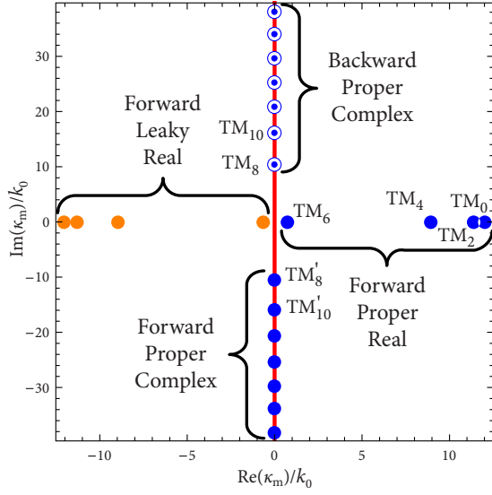
FIG. 6. (Color online) Visualization of the spectrum on the \kappa_m plane. All parameters are the same as in Fig. 4. Proper and leaky modes are shown for forward, \bullet , and backward, \circ , modes. The thick line is the continuous spectrum. The complex modes have a small, yet nonzero, positive real part— which is what makes them proper modes, unlike the continuous part of the spectrum which is improper. Thus complex modes and the continuous spectrum do not intersect.
