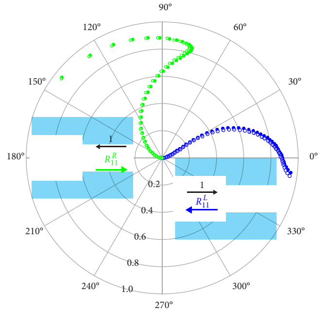
FIG. 13. (Color online) Reflection coefficient of the main mode at the junction between two MIM waveguides of different insulator thicknesses, plotted on the complex plane within the unit circle. Both waveguides have \epsilon_m=-143.497-i9.517 and \epsilon_i=1.0 . Filled circles, \bullet , are FDFD results, empty circles, \circ , are mode-matching results. The left waveguide thickness is fixed at 2a=0.9\lambda . The right waveguide thickness varies from 2a'=\{0.02\lambda, 0.04\lambda, \dots, 0.9\lambda\} . The origin is the zero reflection point that corresponds to a=a' . As a' decreases progressively toward zero, we move progressively along the curves away from the origin. The first set of curves, R_{11}^L , are for the case when the mode of the left waveguide , traveling from left to right, is scattered by the junction. The second set of curves, R_{11}^R , are for the case when the main mode of the right waveguide , traveling from right to left, is scattered by the junction. Insets illustrate the respective cases. Details about the FDFD calculations can be found in Ref. 67.
