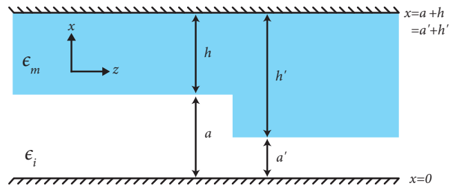
FIG. 8. (Color online) Geometry for mode matching. x = a + h plane of Fig. 8 is terminated by a perfect electric conductor which leads to a discretization of the continuous spectrum.
