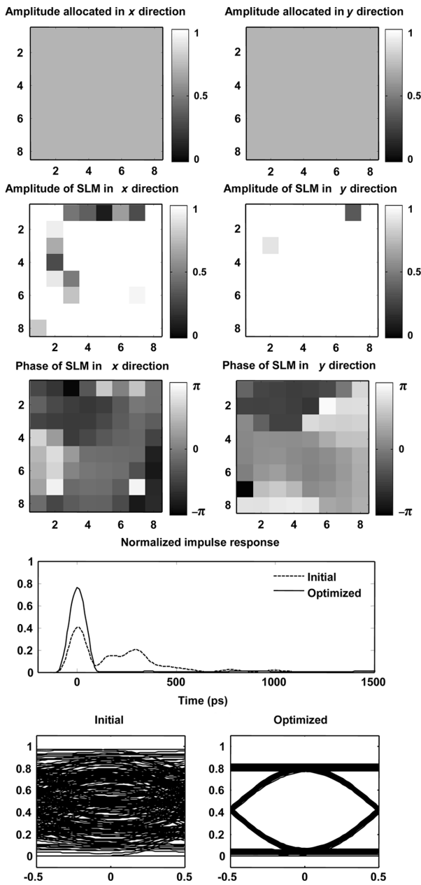
Fig. 5. Configuration C: fixed uniform amplitudes allocated to two SLMs, optimized amplitudes and phases on two SLMs, initial and optimized impulse responses and eye diagrams for a 1-km, 50- \mu m-core graded-index MMF in medium-coupling regime, \sigma_c = 4.62 \text{ m}^{-1} .
