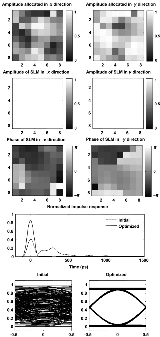
Fig. 7. Configuration E: optimized amplitudes allocated block-wise to two SLMs, optimized amplitudes and phases on two SLMs, initial and optimized impulse responses and eye diagrams for a 1-km, 50- \mu\text{m} -core graded-index MMF in medium-coupling regime.
