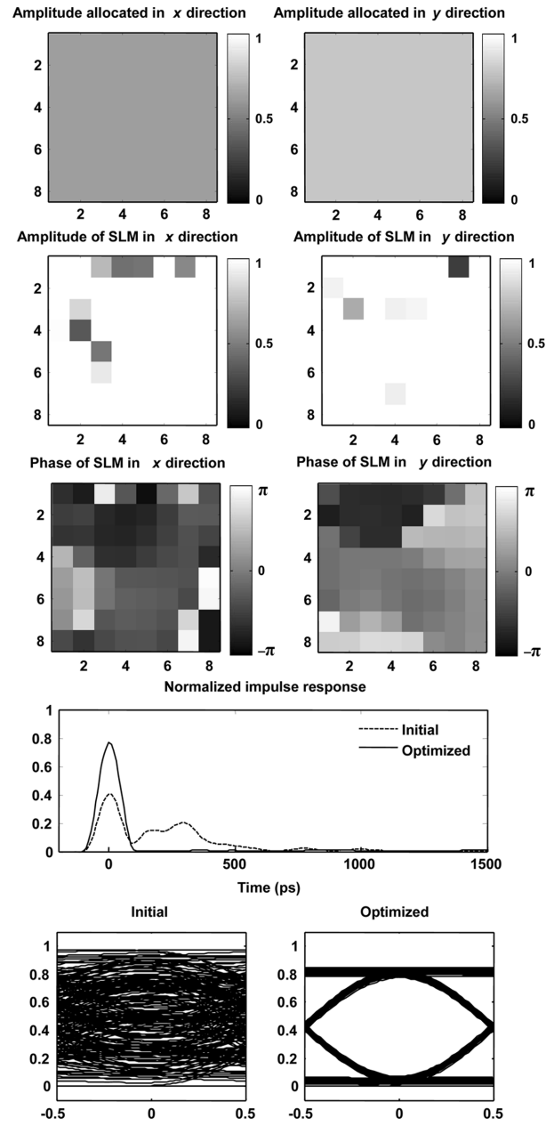
Fig. 6. Configuration D: optimized uniform amplitudes allocated to two SLMs, optimized amplitudes and phases on two SLMs, initial and optimized impulse responses and eye diagrams for a 1-km, 50- \mu m-core graded-index MMF in medium-coupling regime.
