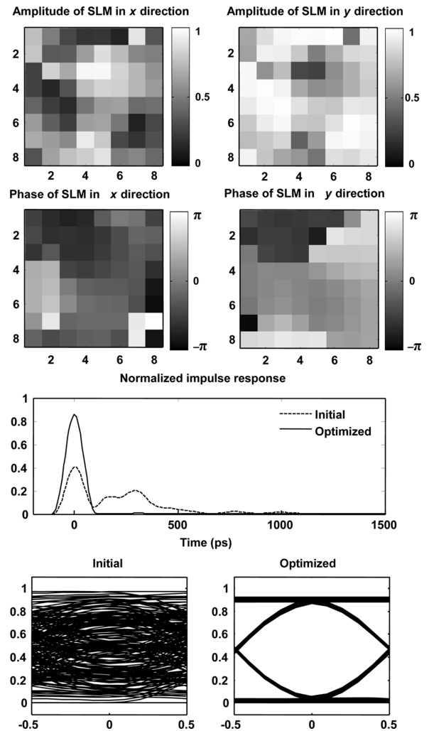
Fig. 4. Configuration B: optimized amplitudes and phases for two polarizations on SLM, initial and optimized impulse responses and eye diagrams for a 1-km, 50- \mu\text{m} -core graded-index MMF in medium-coupling regime.
